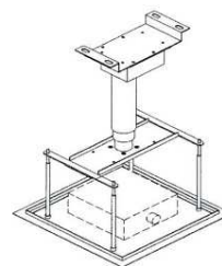
Diagram illustrating the experimental setup for the ceiling effect test. The setup includes a Control Box, an Expansion pillar, a True ceiling, and a False ceiling.
